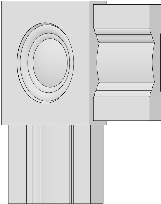
WMB100 Belly Band 1 1/16" x 4-1/4" (shown with rosette)
