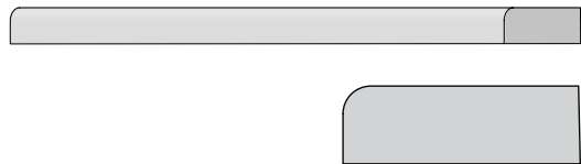
WM888 Flat Stop 3/8" x 1-1/8" x 7/0
