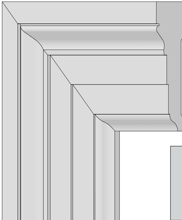
WOC5005 Colonial Revival 1-3/16" x 4-3/8"
