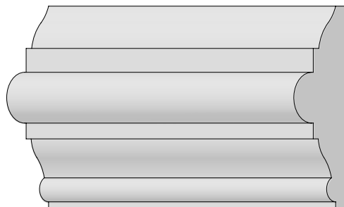
WM300 Williamsburg 1-1/16" x 3"
