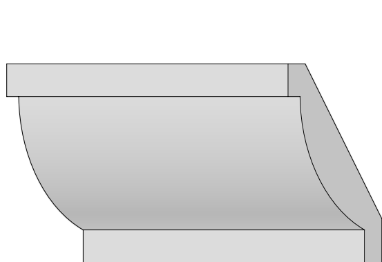
WOCM001 Classical Colonial 3/4" x 3-9/16"
